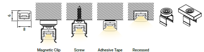
Magnetic Clip
