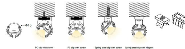
PC clip with screw
