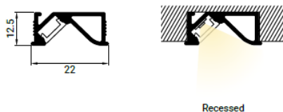
Recessed
