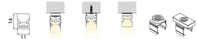
Magnetic Clip Screw Magnetic Tape
