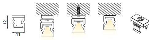
Magnetic Clip Screw Magnetic Tape
